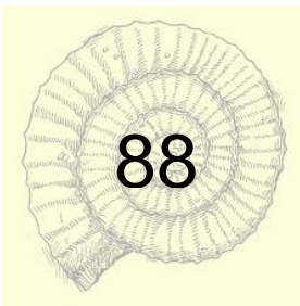
Ammonites
